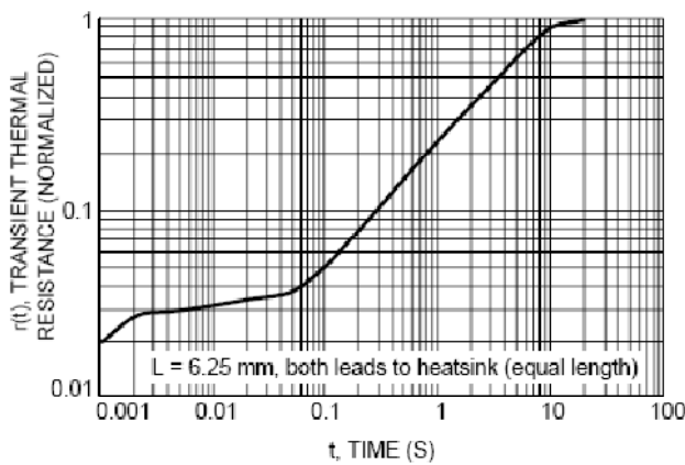
FIG.5 - THERMAL RESPONSE
