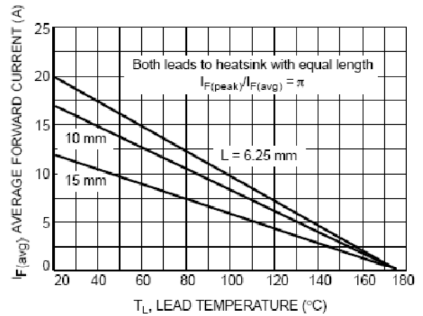
FIG.4 - MAXIMUM CURRENT RATINGS
